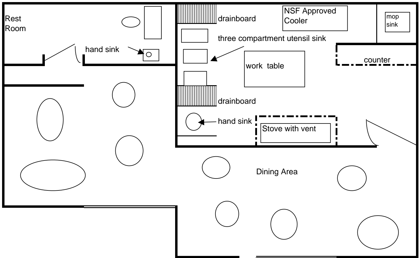
Plot Plan
