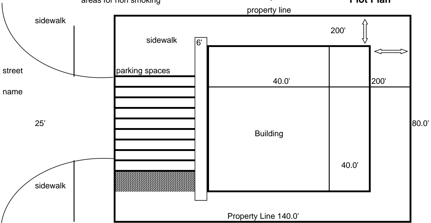
Plot Plan
